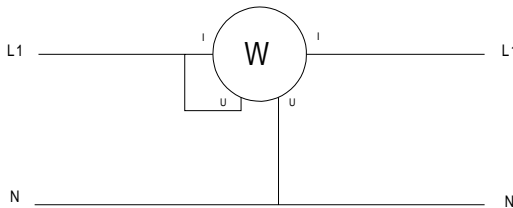
Fig 4.4.1 Single-phase connection diagram
