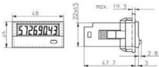
Dimensions CODIX 140 and 142
