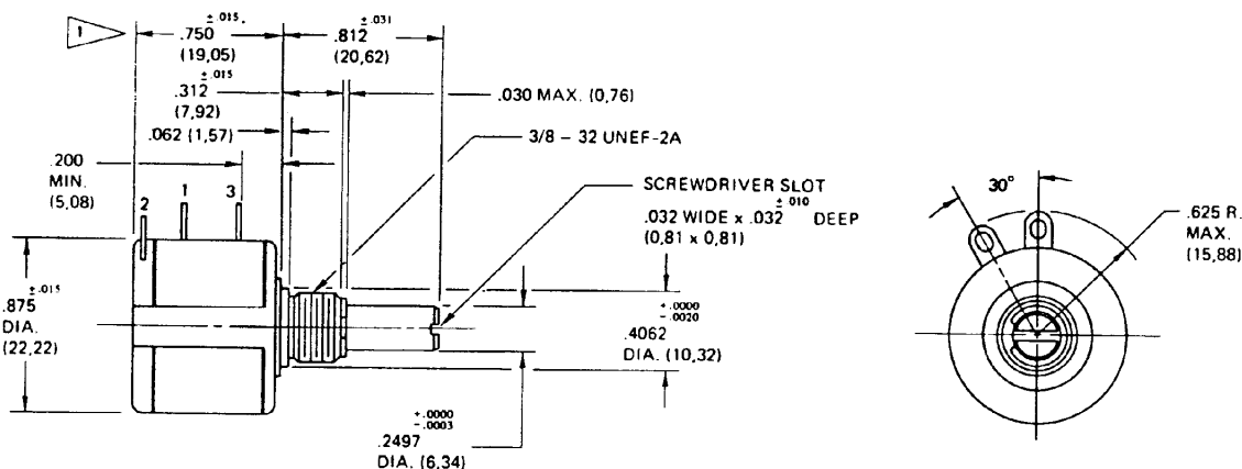
BUSHING MOUNT
