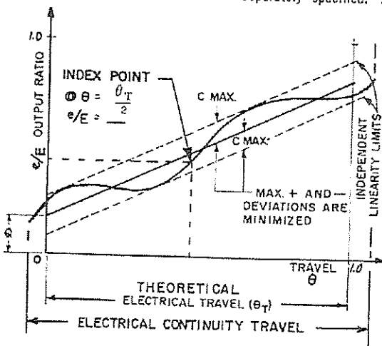
FIGURE 5.8.2 Independent linearity — nonwirewound
