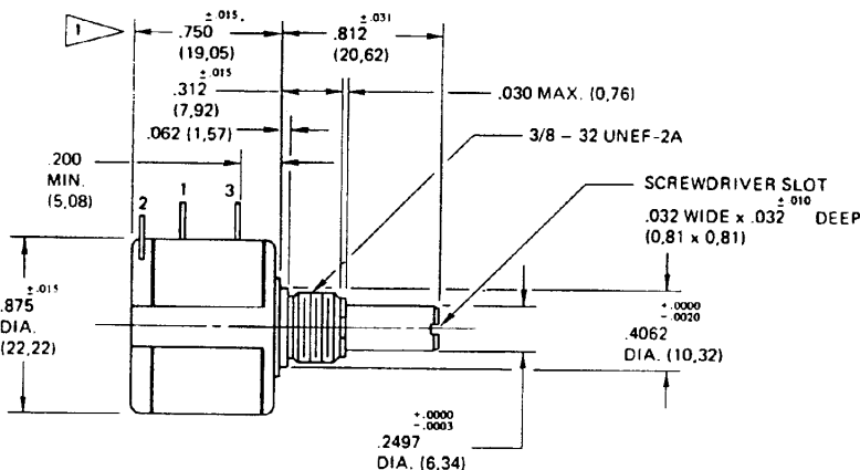
BUSHING MOUNT
