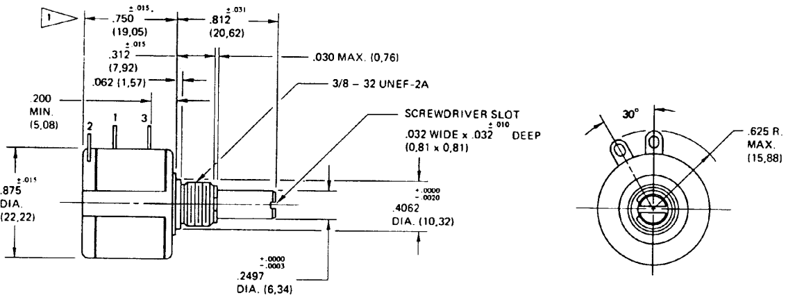
BUSHING MOUNT
